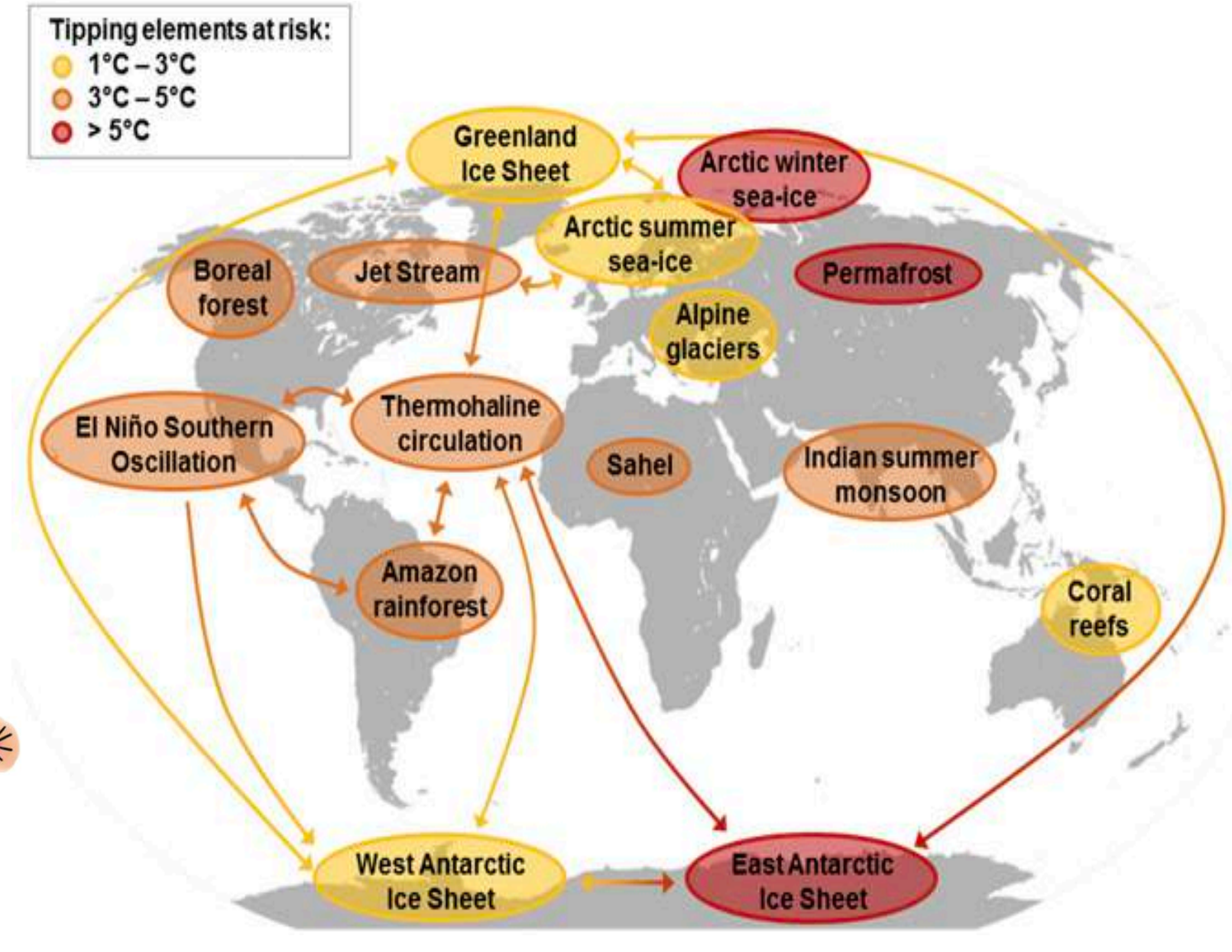
Figure 3. Earth's tipping points Map of the locations of potential large-scale tipping points, the estimated temperature ranges of the tipping points and potential interactions between tipping points. Crossing one tipping point can increase the risk of crossing another (PNAS 2018 Steffen et al. 8 )
